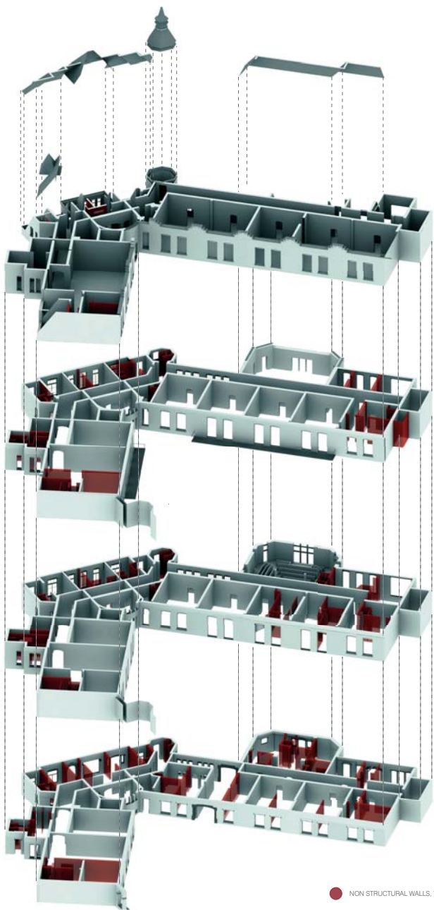
EXPLODED VIEW OF EXISTING BUILDING
